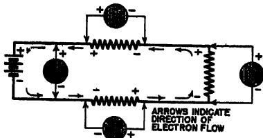
CORRECT CONNECTIONS FOR VOLTAGE MEASUREMENTS
